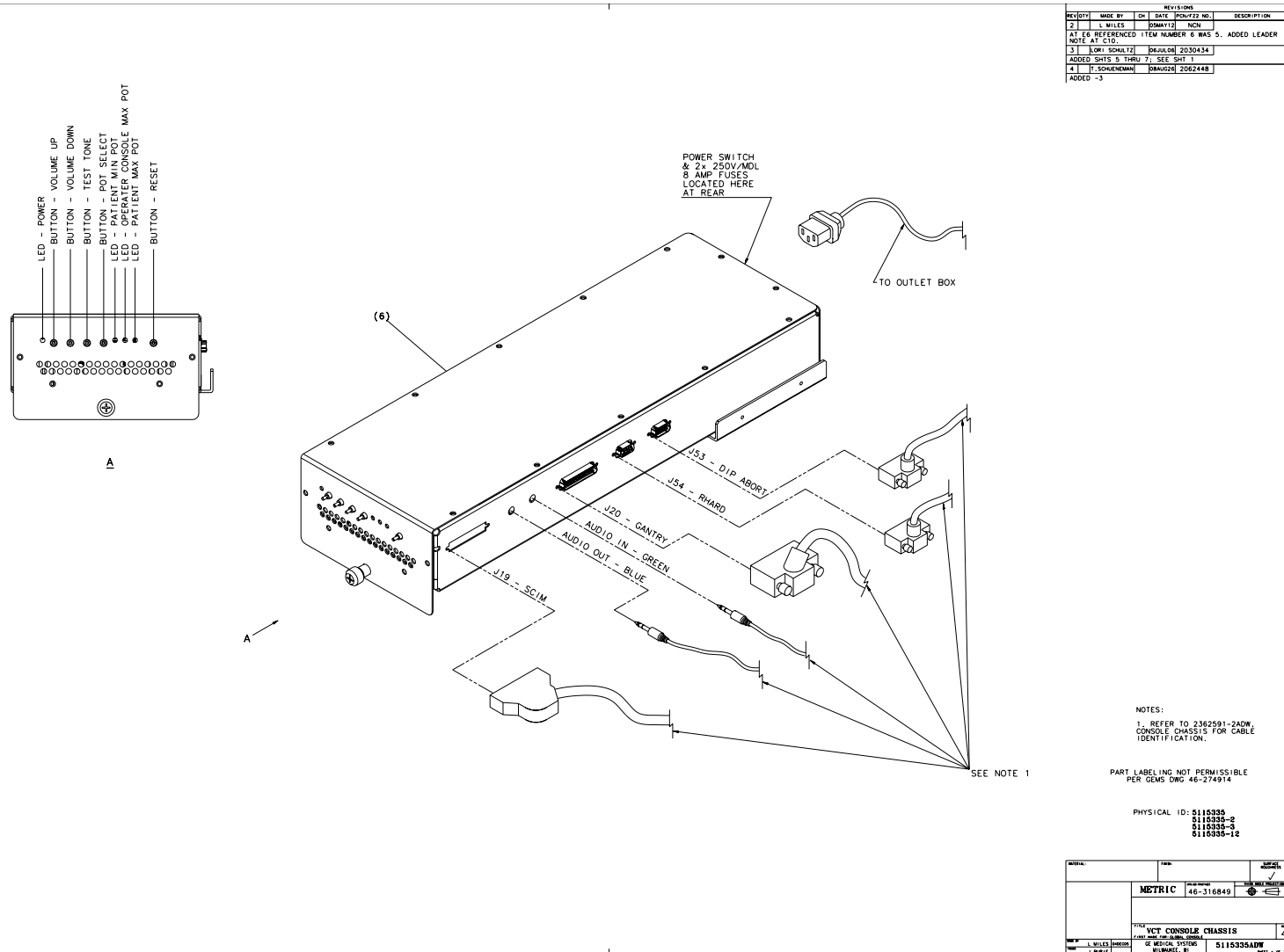
Figure 1-12 GOC5 (5115335 Sheet 4, Rev 8)
