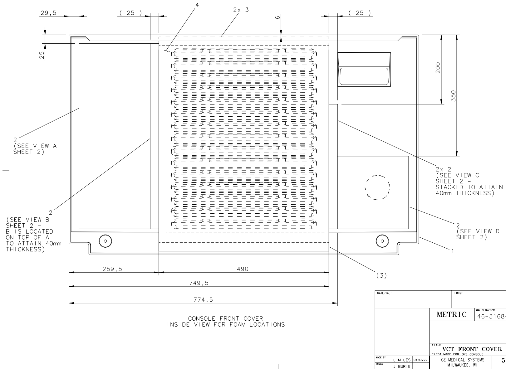
Figure 1-18 Cover Assy - Console Front (5128181 Sheet 1, Rev 1)
