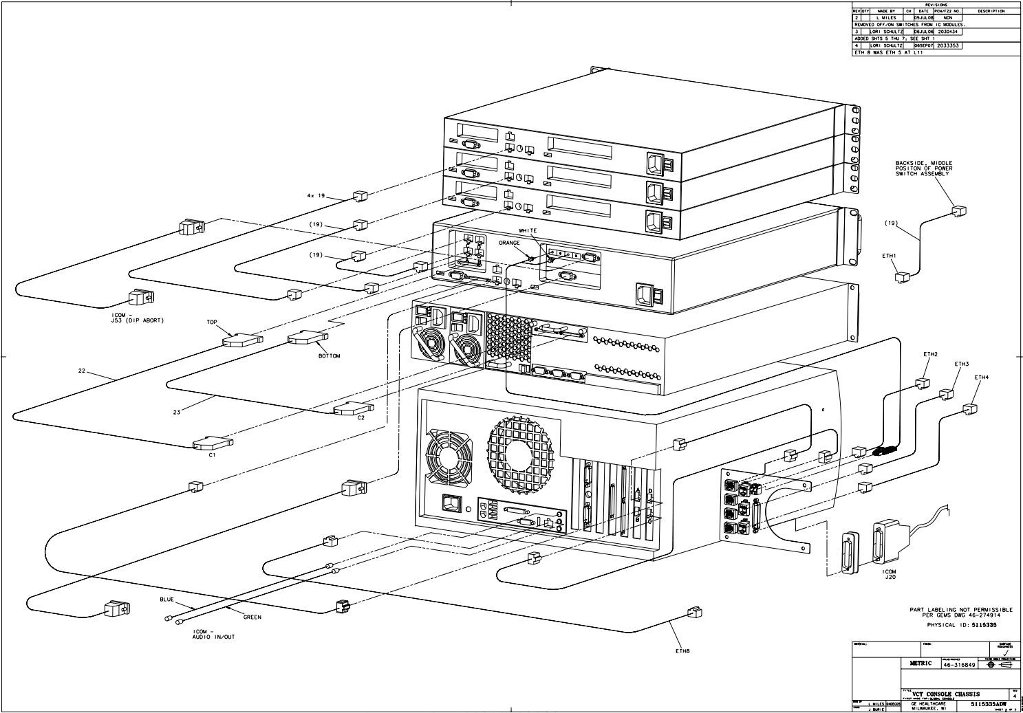
Figure 1-2 GOC5 (5115335 Sheet 2, Rev 8)
