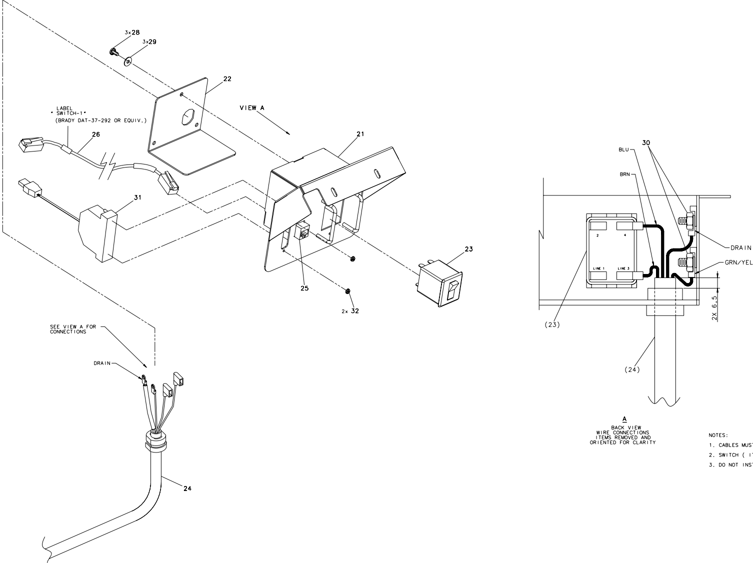
Figure 1-16 SubAssy, Power Distribution Switch Panel - VCT (5122587 Sheet 2, Rev 7)
