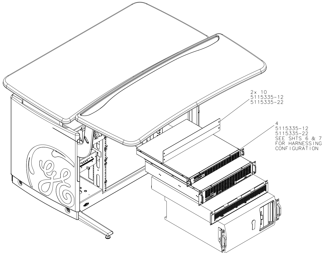
Figure 1-5 GOC5 (5115335 Sheet 5 - Partial, Rev 8)
