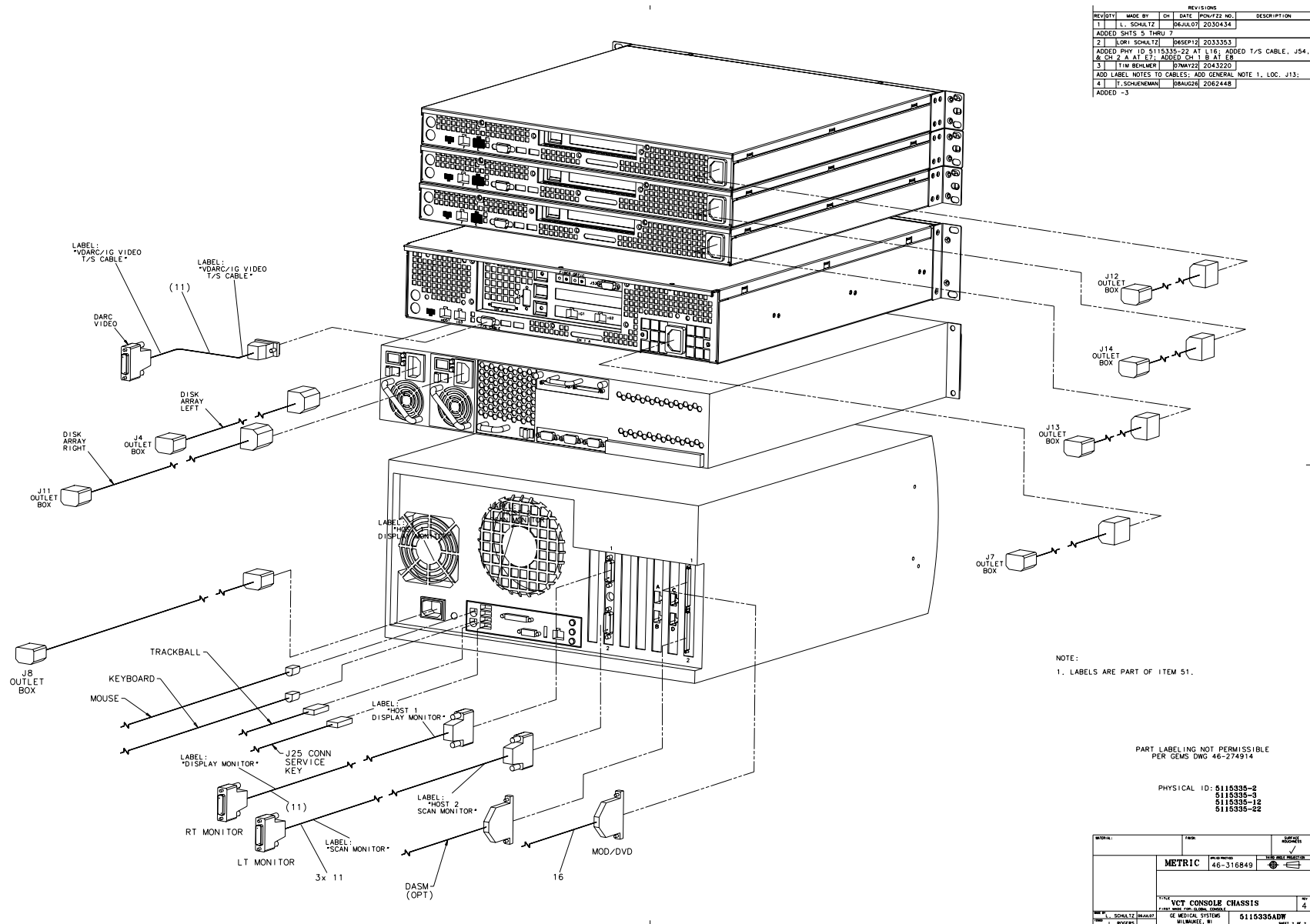
Figure 1-7 GOC5 (5115335 Sheet 7, Rev 8)
