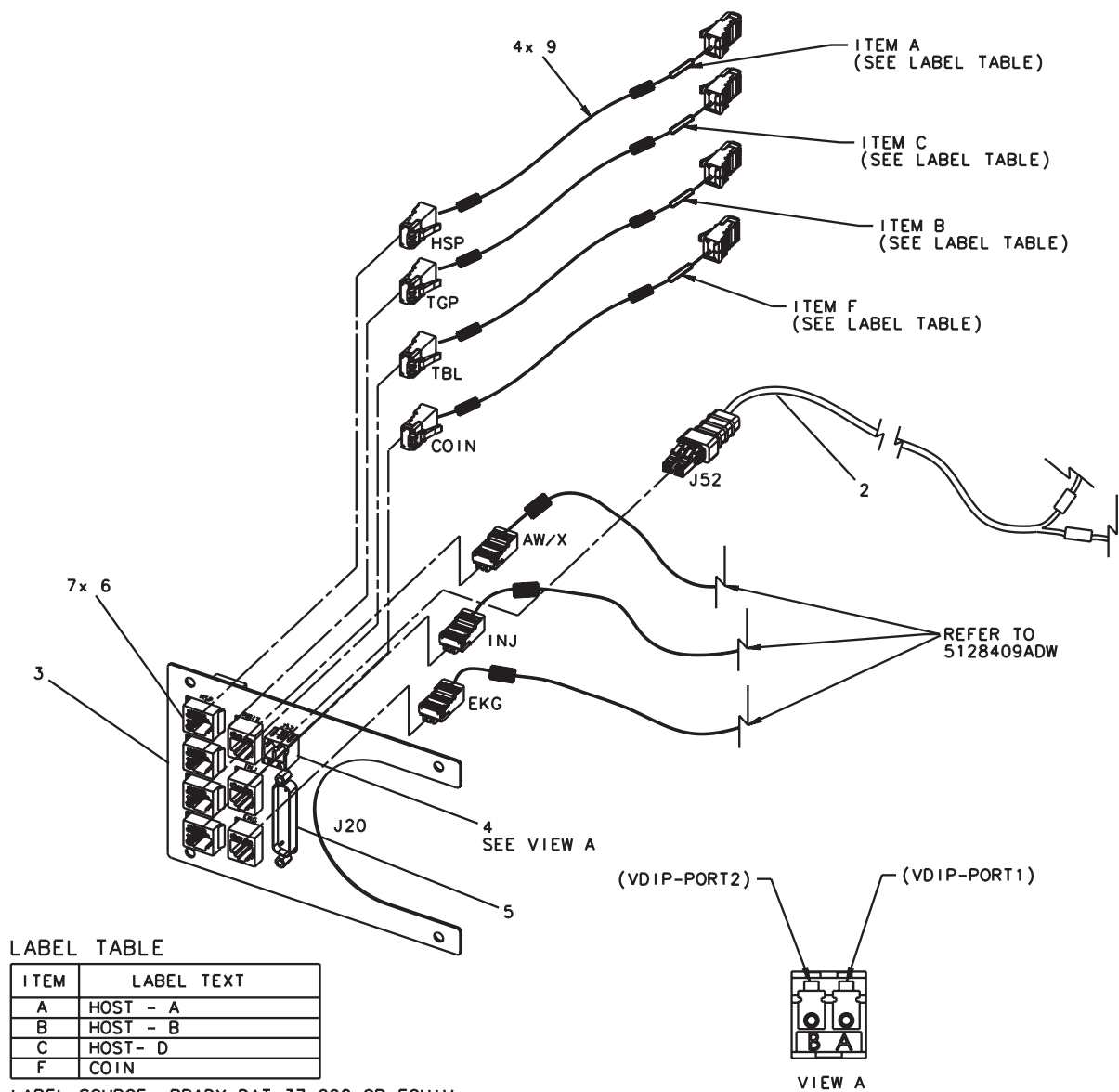
Figure 1-17 SubAssy, Console Rear Bulkhead Panel - VCT (5122506 Sheet 1, Rev 5)
