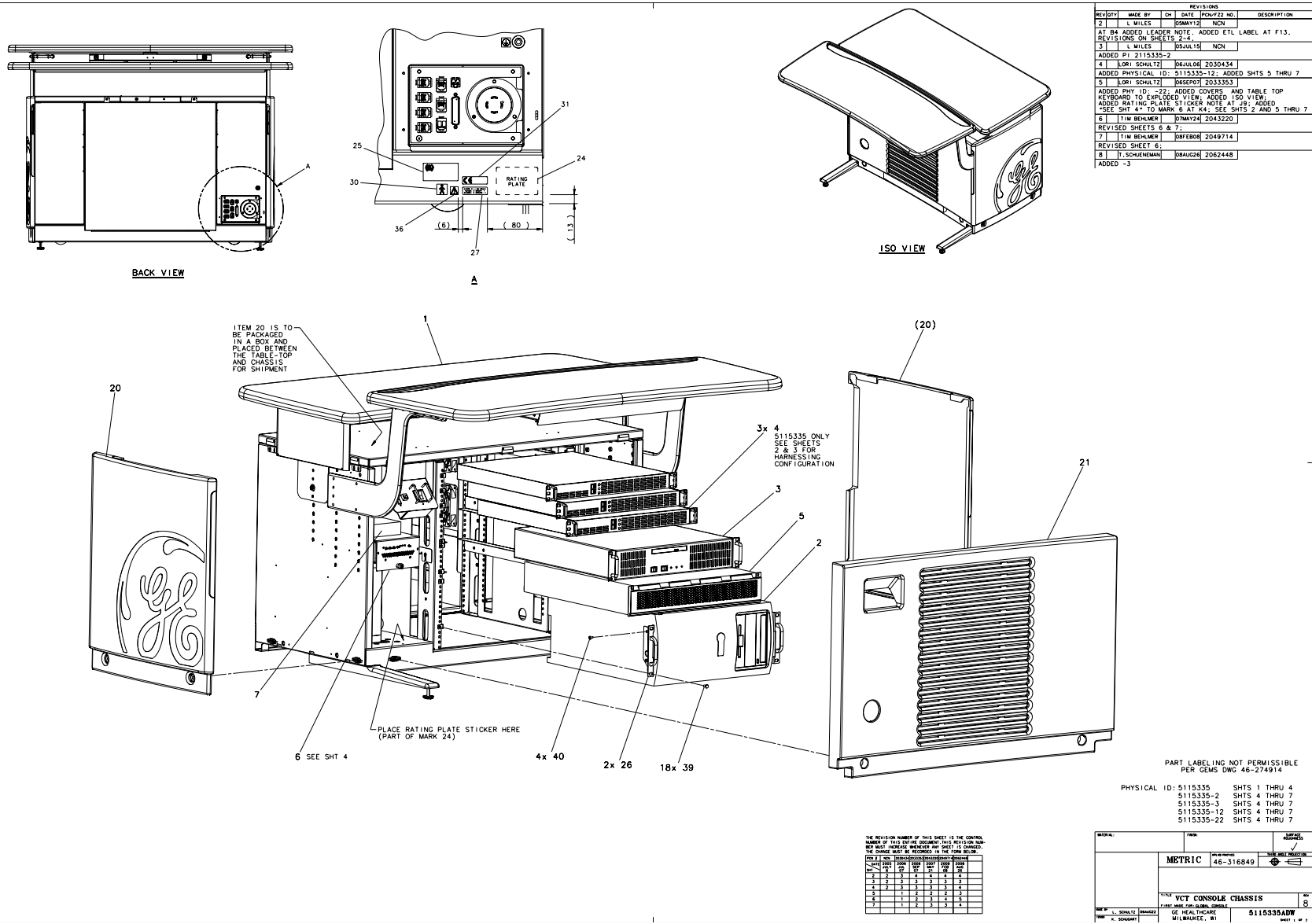
Figure 1-1 GOC5 (5115335 Sheet 1, Rev 8)
