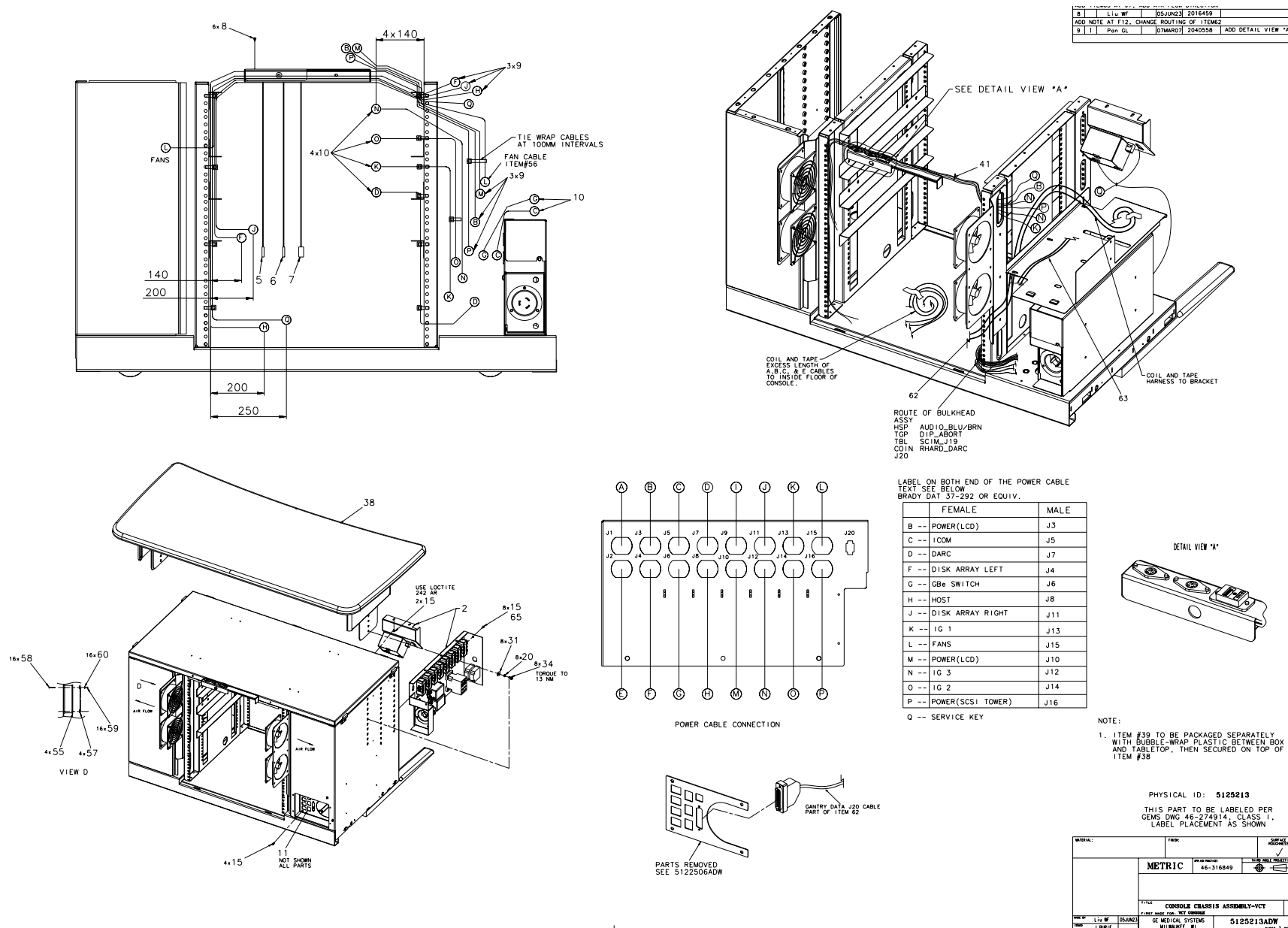
Figure 1-14 Console Chassis Assy - GOC5 (5125213 Sheet 2, Rev 9)
