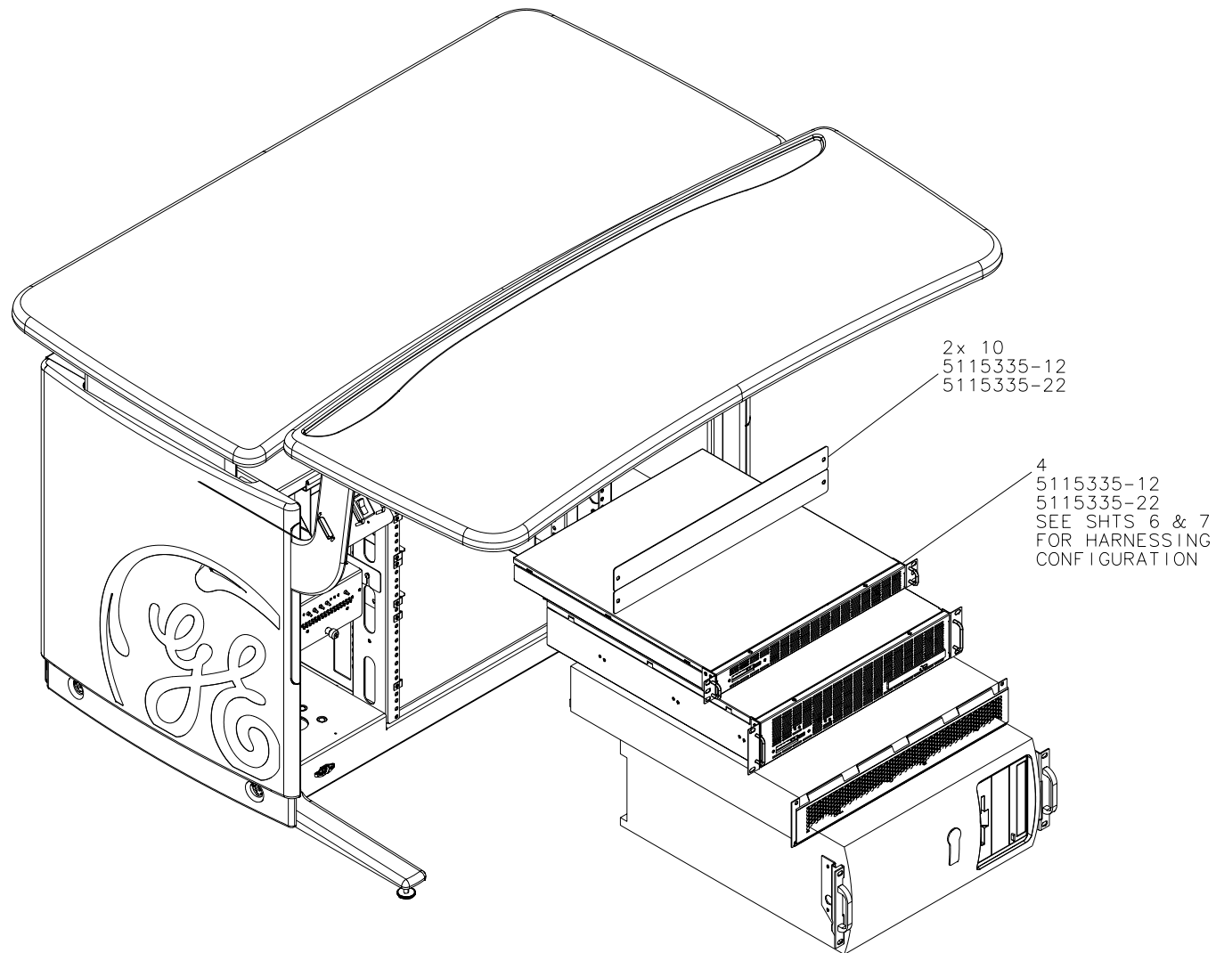
Figure 1-9 GOC5 (5115335 Sheet 5 - Partial, Rev 8)
